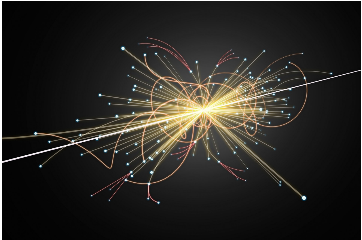
ABOVE, PARTICLE COLLISION VISUALIZATION OF ONE CERN LARGE HEDRON COLLIDER'S 'BILLIONS OF DOLLARS' WORTH OF EXPERIMENTS.
