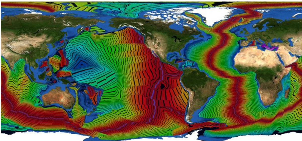
ABOVE, MAP VISUALIZING OCEAN FLOOR RATES OF EXPANSION, PUSHING FROM FASTER VOLCANIC (RED) TO SLOWER (BLUE) ZONES. *11
